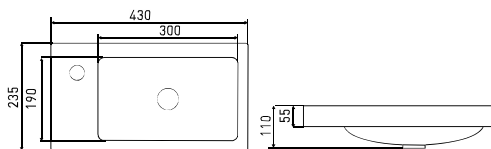
KR 120 TWIN
