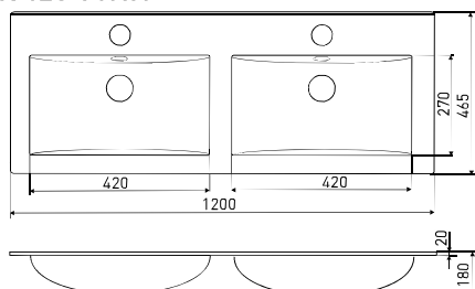
KR 120 TWIN
